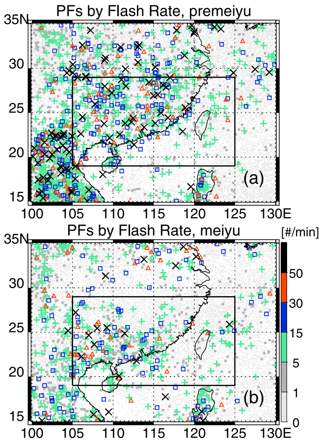
Figure 2. Distribution of precipitation features categorized by lightning flash rate during preseason and Mei-Yu. Values of flash rate (#/min) are indicated by different colors. Markers present features with different flash rate, the values of which are presented according to the colors in the color bar.
