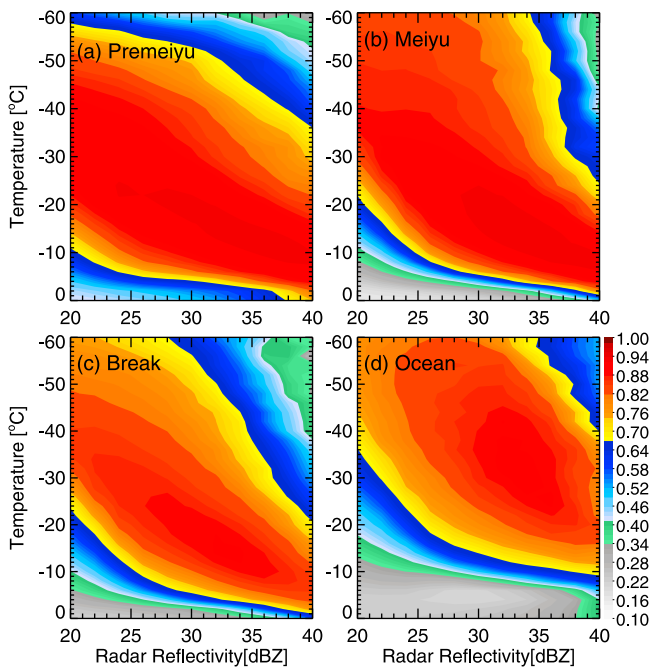
Figure 7. Linear correlation coefficients between lightning flash rate and area of radar reflectivity for land features during (a) pre-mei-yu, (b) Mei-Yu, and (c) Break, and (d) for systems in all periods over ocean.
